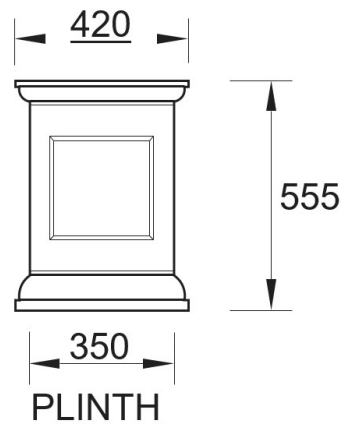
Plinth Pedestal
